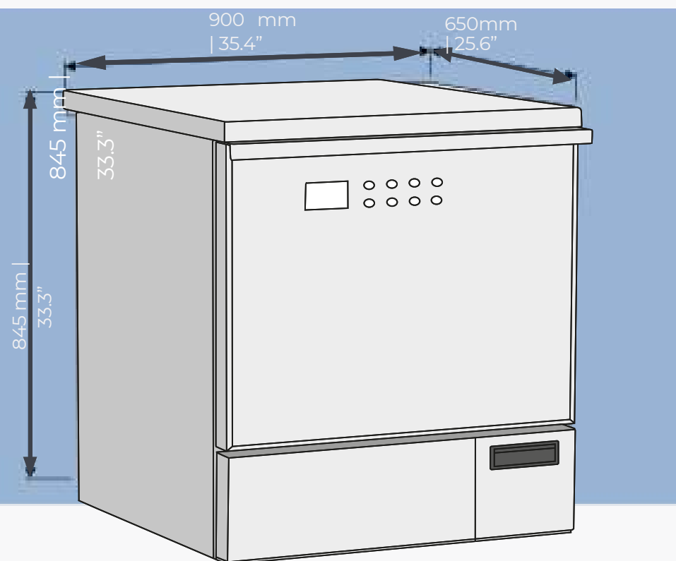
Dimensions machines
